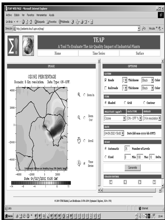
Figure 6. O 3 power plant concentrations impact at 15h00 on September, 4, 2002 for the 3 km spatial resolution model domain showing the areas with increase and decrease on O 3 concentrations due to the emissions from the power plant.
