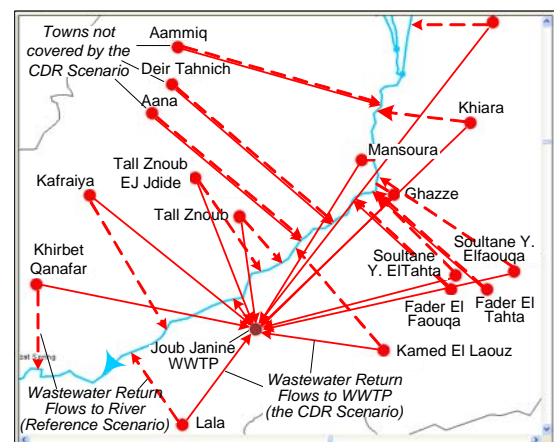
Figure 5. A snapshot of the ULB DSS simulation environment.
