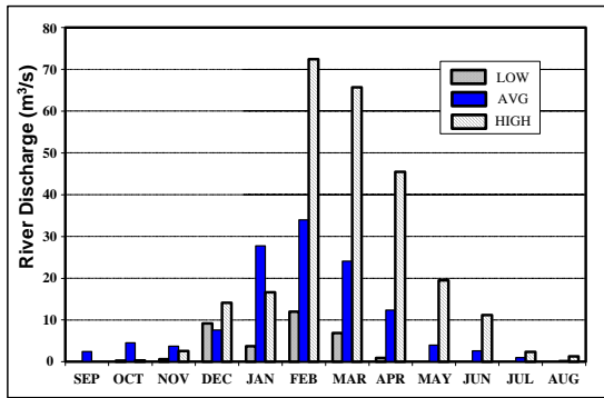
Figure 6. Monthly discharges for the selected water years.
