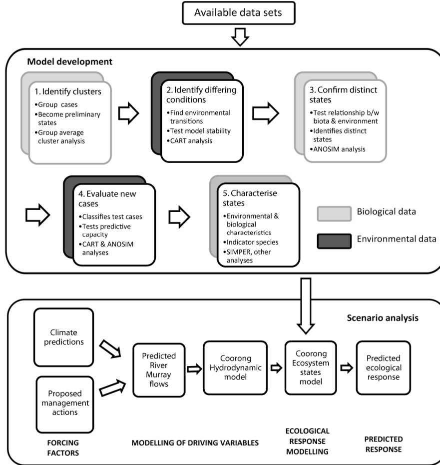
Figure 1. Flow chart describing the model development process and how the ecosystem states model can be used in combination with other existing models for the region to run various scenario analyses, including the generic steps (shown in upper case) that could be followed in applying this method to other case studies or disciplines.
