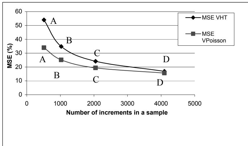
Figure 5. The Mean Squared Errors (MSE's) of V_{HT} and V_{Poisson} expressed as a percentage of the sample-to-sample variance of c_{sample} for the scenarios studied during the second computer experiment. Virtual population = rok10. The sampling modes are: A = ( N_{Block}=16 , n=2 ), B=( N_{Block}=16 , n=4 ), C=( N_{Block}=16 , n=8 ), and D=( N_{Block}=16 , n=16 ).
