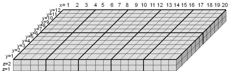
Figure 1. Model of the population. In the here-depicted model z ranges from 1 to 2; y ranges from 1 to 12; x ranges from 1 to 20; and the population is divided in 10 equally-size blocks. The models that are used here are significantly larger (and therefore more realistic).
