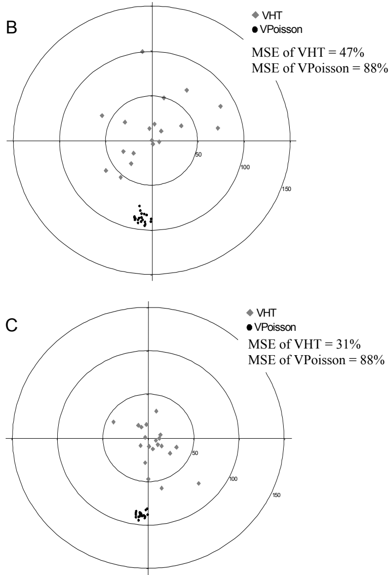
Figure 7. The errors (expressed as a percentage of V(c_{\text{sample}}) ) of V_{\text{HT}} and V_{\text{Poisson}} for the same virtual population and sampling modes A, B and C as in Figure 4. The distance of a point to the origin represents the magnitude of the error. Hence the analogy with a dart board: a point at the origin means that no error is made when the corresponding sample and estimator are used to estimate the variance. Three circles are depicted for each “dart board”: a circle indicating the region with error=50%, 100% and 150%. As the number of increments per sample increase going from A to C, the scatter of V_{\text{HT}} becomes more centered in a region close to the origin.
