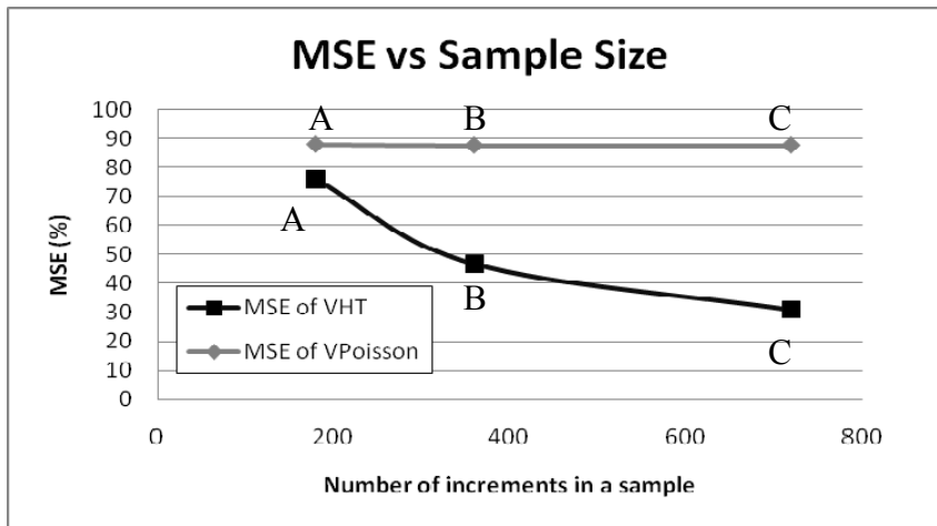
Figure 4. The Mean Squared Errors (MSE's) of V_{HT} and V_{Poisson} expressed as a percentage of the sample-to-sample variance of c_{sample} for the scenarios studied during the second computer experiment. Virtual population = gas01. The sampling modes are: A = ( N_{Block}=16 , n=2 ), B=( N_{Block}=16 , n=4 ), C=( N_{Block}=16 , n=8 ).
