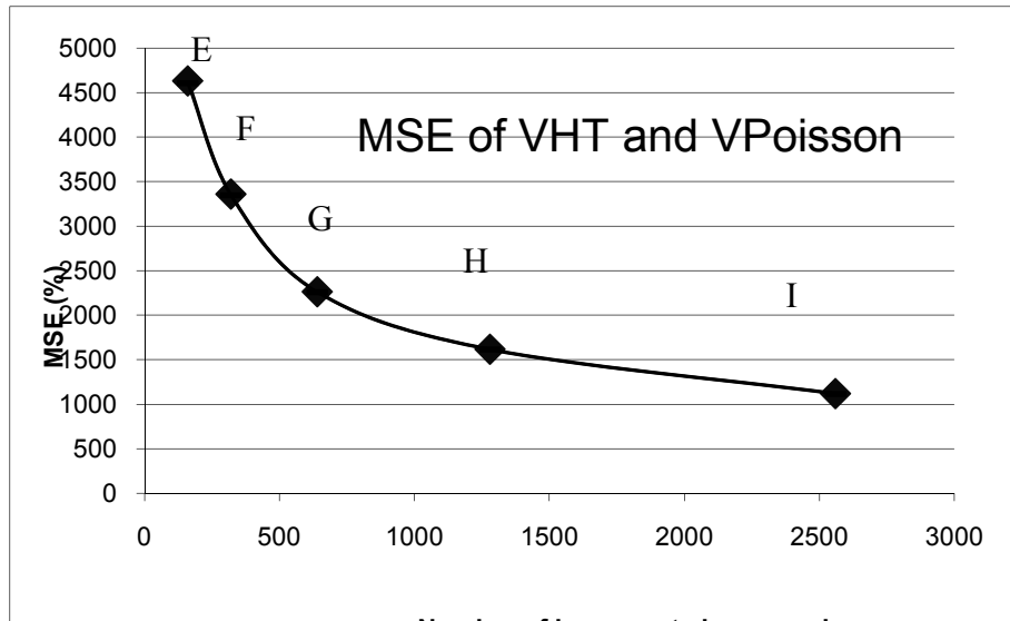
Figure 6. The Mean Squared Errors (MSE's) of V_{HT} and V_{Poisson} expressed as a percentage of the sample-to-sample variance of c_{sample} for the scenarios studied during the second computer experiment ( V_{HT} and V_{Poisson} resulted in almost identical values of MSE). Virtual population = dpa03. The sampling modes are: E = ( N_{Block}=1, n=10 ), F=( N_{Block}=1, n=20 ), G=( N_{Block}=1, n=40 ), H=( N_{Block}=1, n=80 ) and I=( N_{Block}=1, n=160 ).
