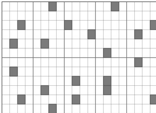
Figure 2. Schematic depiction of the sampling design. This is a top view of the same virtual population as in Figure 1. The grey squares represent the vertical stacks of increments that are part of a random sample. In the here-depicted scenario, the population is divided into 10 equally-sized blocks and from each block two vertical stacks of increments are selected
