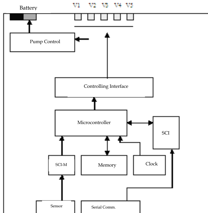
Figure 3. Basic scheme of the plate circuit equipment hardware.
