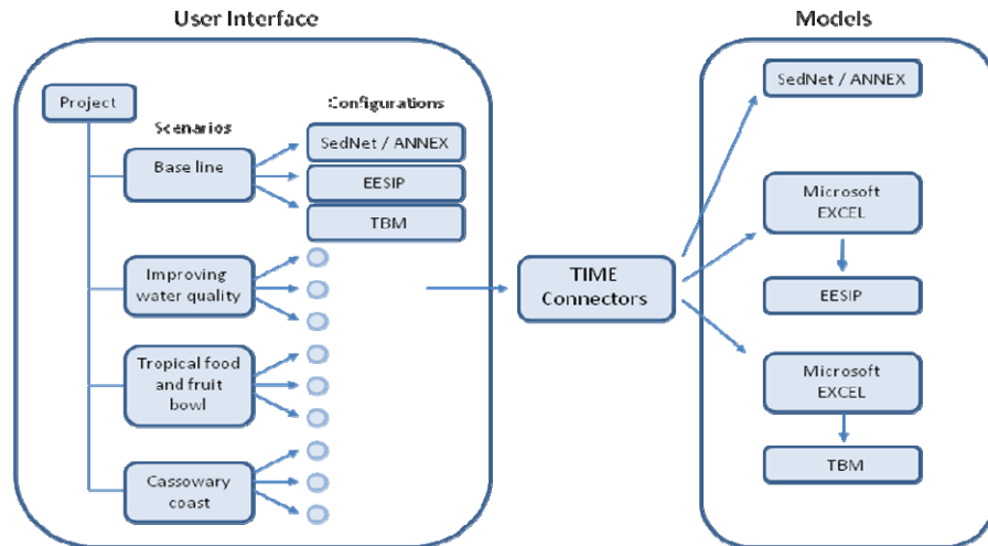
Figure 1. Schematic representation of the Landscapes Toolkit depicting the separation between the user interface and the external models. The Baseline scenario and associated datasets and functionalities form the central part of the Landscapes Toolkit, which support participatory development of future scenarios (e. g. Improving water quality/Tropical food and fruit bowl/Cassowary coast). The water quality (SedNet/ANNEX), economic (EESIP) and biodiversity (TBM) models are the component models linked in the Landscapes Toolkit. TIME based connectors [Rahman et al. 2004] have been created to act as the glue between the user specified scenario configurations and the models [Source: Bohnet et al. in review].
