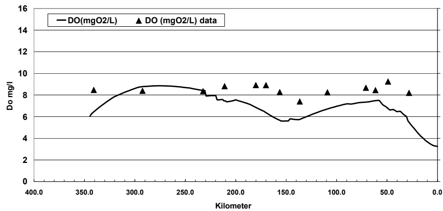
Figure 2- DO concentration (mg/l) January 2003 (Calibration )
