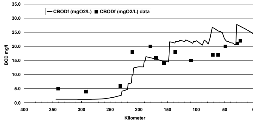
Figure 5- BOD concentration (mg/l) August 2004 (Validation)
