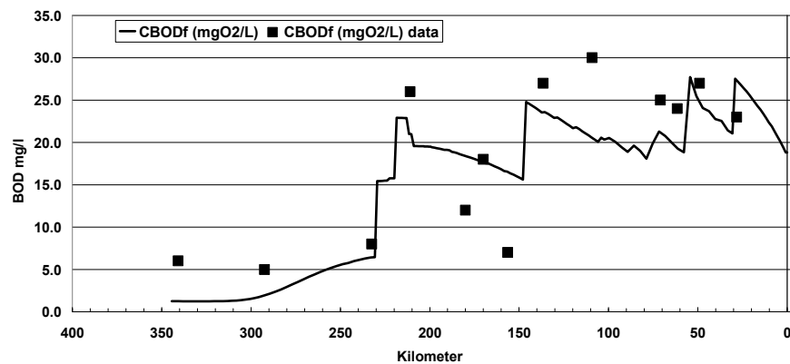
Figure 3- BOD concentration (mg/l) January 2003 (Calibration )
