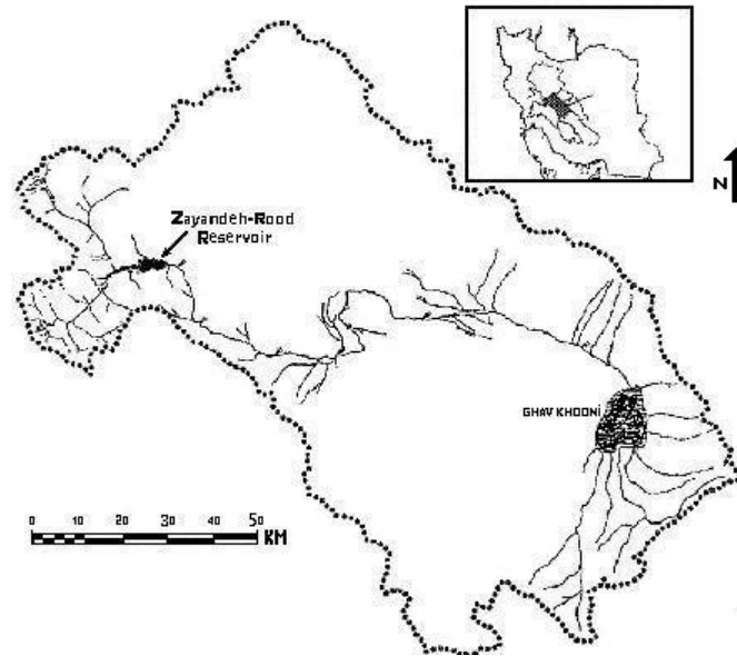
Figure 1- The Zayandehrood River location and drainage area
