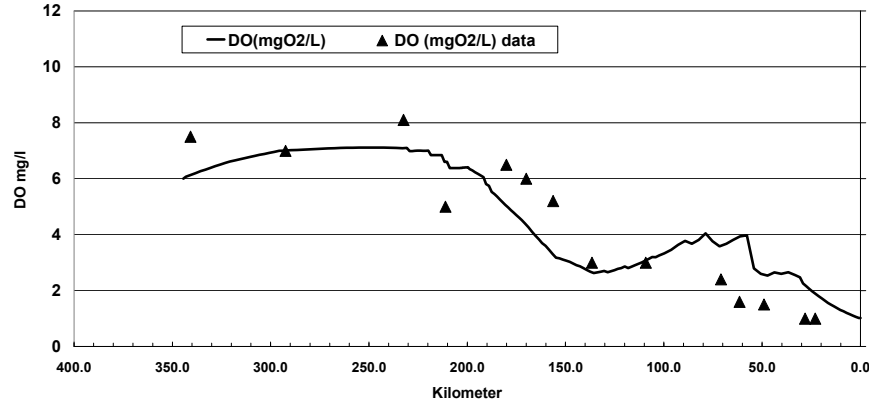
Figure 4- DO concentration (mg/l) August 2004 (Validation)
