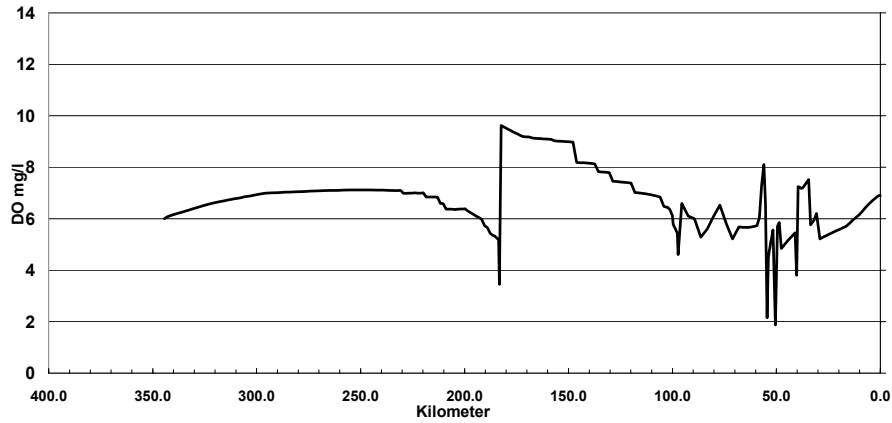
Figure 6- DO concentration with 20% increase of loads and local oxygenation
