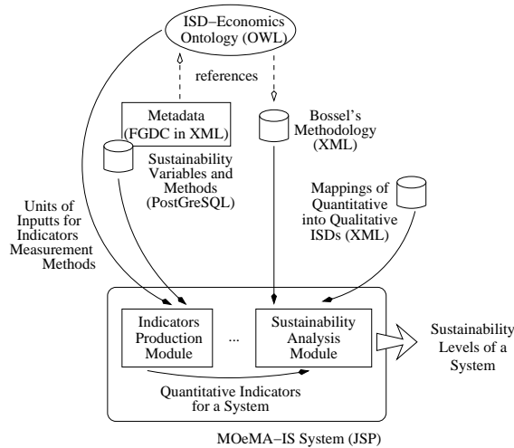
Figure 3: The MOeMA-IS framework.
