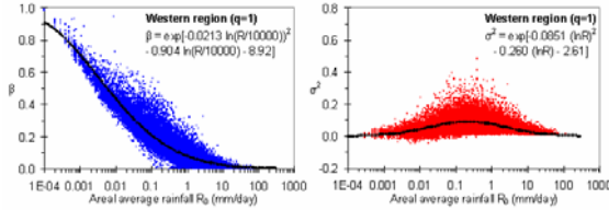
Figure 4. Relationships between the cascade parameters and western regional average rainfall.
