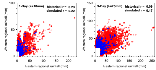
Figure 6. Spatial correlations of historical (solid) vs. generated (hollow) regional rainfall for July.
