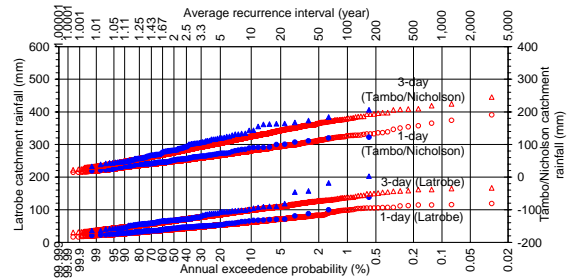
Figure 7. Typical AEP plots of historical (solid) vs. simulated (hollow) catchment average rainfall.
