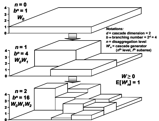
Figure 3. Schematic of a 2-d construction of discrete multiplicative random cascades.
