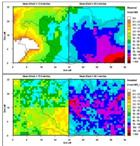
Figure 8. Typical observed and simulated daily spatial rain fields of a moderate/heavy rainfall day.
