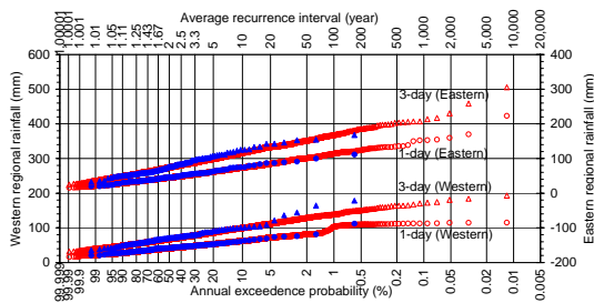
Figure 5. AEP plots of historical (solid) vs. generated (hollow) regional average rainfall.
