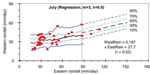
Figure 2. Relationship between eastern and western regional average rainfall for July.
