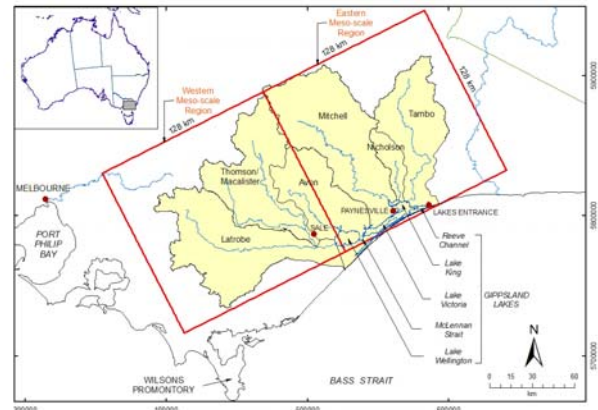
Figure 1. The Gippsland Lakes catchments with two meso-scale square regions.
