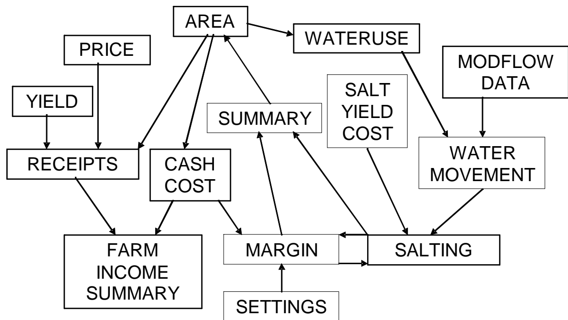
Figure 1. ICHAM flowchart
