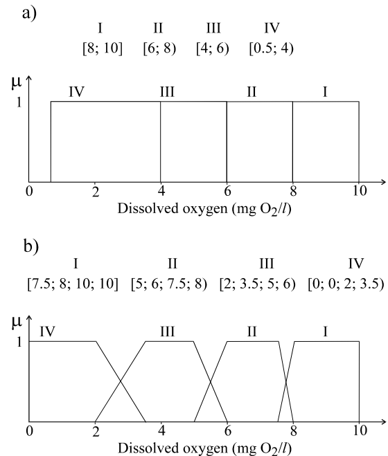
Figure 1. Water quality classes for dissolved oxygen concentrations: a) standard YU classification, b) fuzzy YU classification
