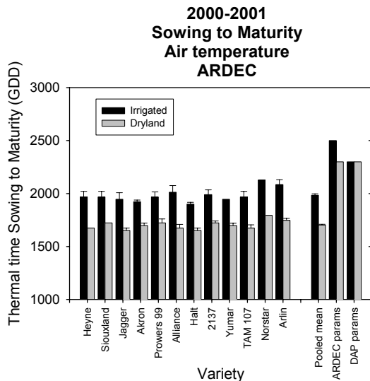
Figure 2. Observed thermal time from sowing (with 1 SE bar) to maturity for 2000-2001 at ARDEC for dryland and irrigated treatments compared to parameter used for simulation. Simulated values are the two rightmost sets of bars. Thermal time uses air temperature for calculating growing degree-days with 0°C base temperature.
