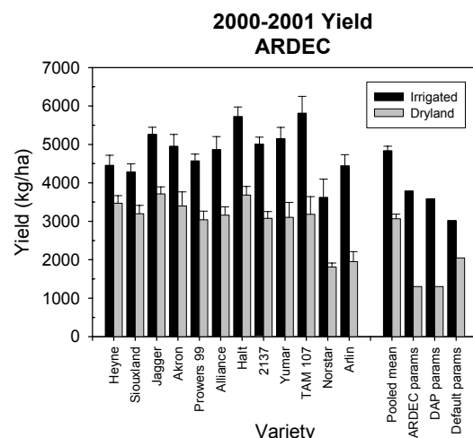
Figure 4. Observed grain yield (with 1 SE bar) for 2000-2001 at ARDEC for dryland and irrigated treatments compared to simulated grain yield for different parameter data sets. Simulated values are the three rightmost sets of bars.
