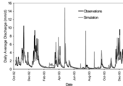
Figure 2: Daily hydrograph Harraby Green catchment – independent simulations
