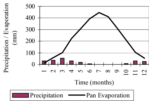
Figure 5. Five year average monthly precipitation and evaporation data.
