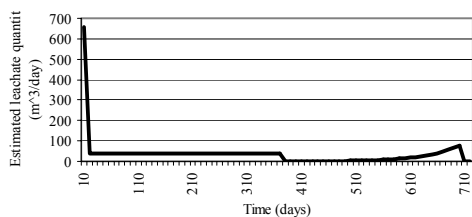
Figure 4. Estimated leachate quantity for a single cell excluding infiltration/evaporation.
