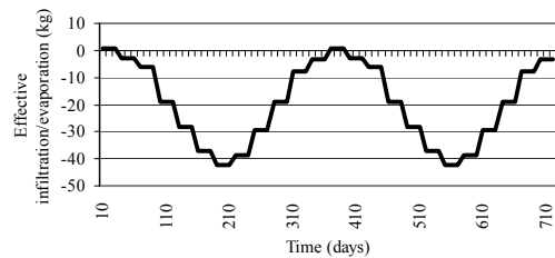
Figure 6. Water gain/loss due to infiltration/evaporation, during the single cell modelling time.
