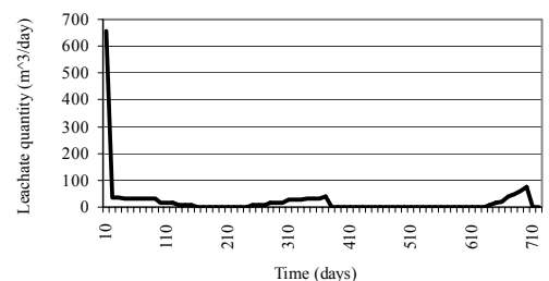
Figure 7. Leachate quantity estimated for a single cell including infiltration/evaporation.
