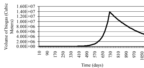
Figure 1. Temporal pattern of biogas generation for a single cell
