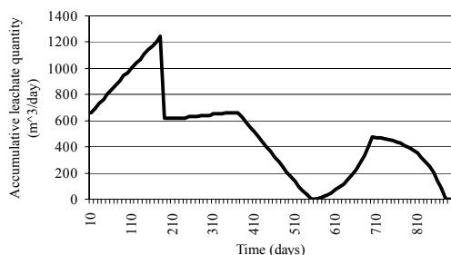
Figure 8. Accumulative leachate generation for a six month operating trench at Kahrizak landfill site.
