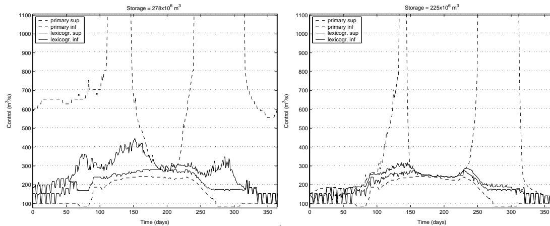
Figure 6: Sections of the optimal control set before and after lexicographic optimization.
