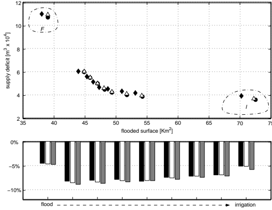
Figure 4: Results of lexicographic optimization.
