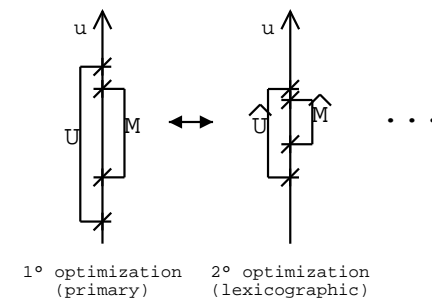
Figure 1: In the lexicographic scheme policy M is used to generate the control set \hat{U} which in turn generates policy \hat{M} and so on.
