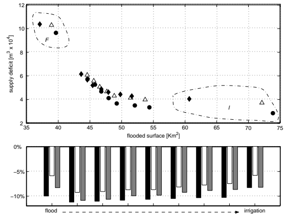
Figure 3: Results of primary optimisation.
