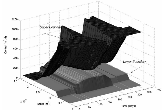
Figure 5: Optimal set controls for primary optimisation.
