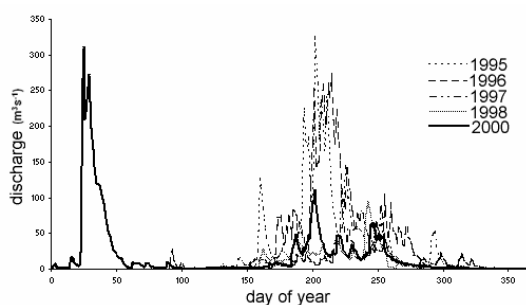
Figure 2. Comparison of watershed inflow to the Swan River in 2000 with more typical years.
