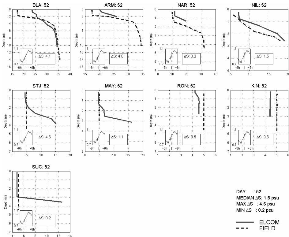
Figure 4. Field versus model (ELCOM) salinity profiles, day 52 (21 February 2000). Insets and key as for Figure 3.
