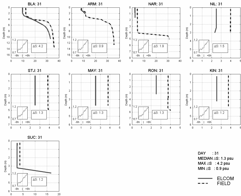
Figure 3. Field versus model (ELCOM) salinity profiles, day 31 (31 January 2000). BLA = Blackwell Reach; ARM = Armstrong; NAR = Narrows; NILE = Nile St; STJ = St Johns; MAY = Maylands; RON = Ron Courtney Island; SUC = Success Hill (see Fig. 1). Insets show tidal height at Fremantle around the time of the measurements. \Delta S is the sum of the squares of the difference between field and model values.
