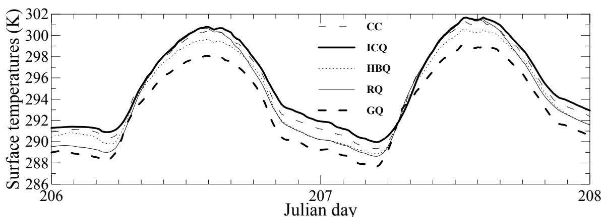
Figure 2. Simulated surface temperatures of: City Centre (CC), Residential Quarter (RQ), Green Quarter (GQ), Industrial-commercial Quarter (ICQ) and High Building Quarter (HBQ).
