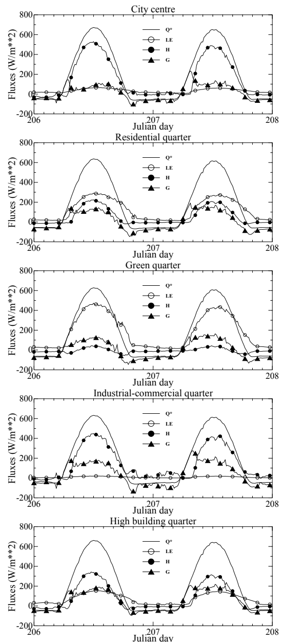
Figure 1. Components of energy balance of each quarter: net radiation ( Q^* ), latent heat flux (LE); sensible heat flux (H) and energy storage (G).
